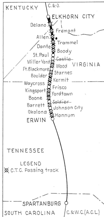
Fig. 1—Map of C.T.C. territory
