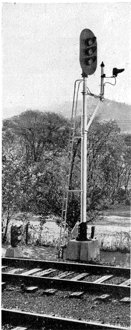
Main-track station-leaving signal on far side of the siding using doll bracket mast with blue marker lamp
